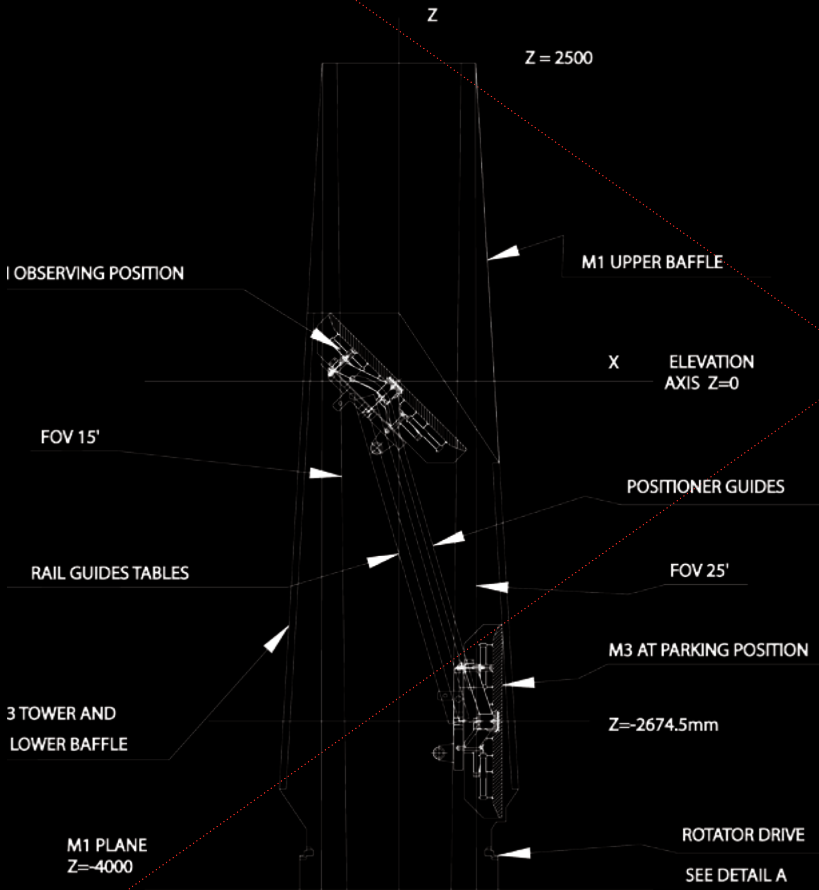
TERTIARY MIRROR TOWER ASSEMBLY
