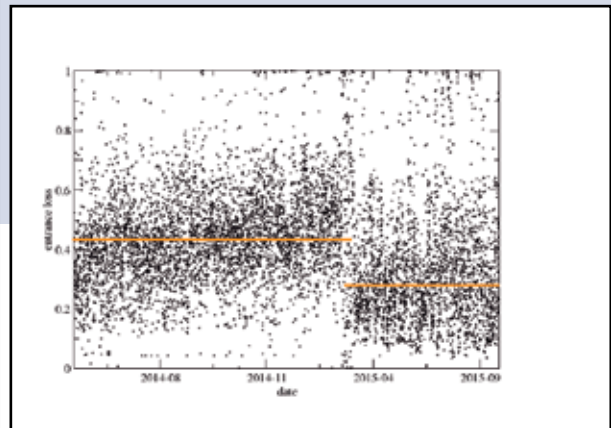
Efficiency of the new STELLA-II/SES guiding algorithm. The fibre entrance light loss was lowered from 43% to 27%.
